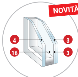
Vetrata INFINITY*
